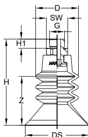
HSE55 External thread
